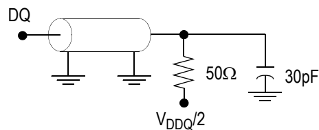
JTAG Port AC Test Load
