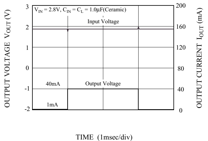
Fig. 6 Load Transient Response ( I_{OUT} = 40\text{mA} )
