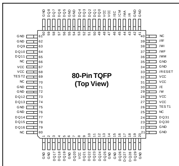
Pinout Diagram
