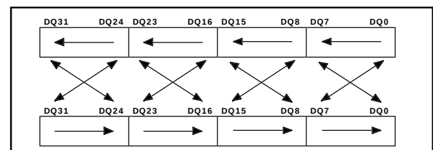
Figure 2: IEEE 802.3/802.5 Format Mapping
