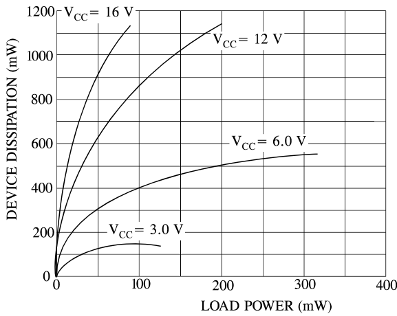
Figure 3. DEVICE DISSIPATION 16 Ω LOAD
