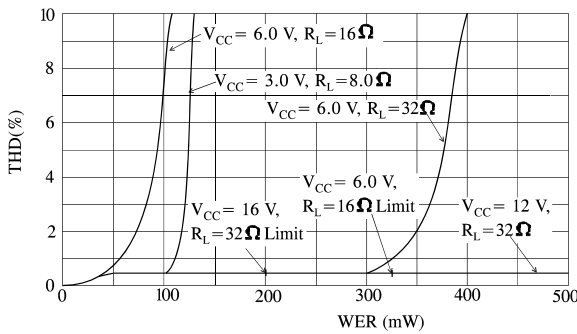
Figure 7. DISTORTION versus POWER f = 1, 3.0 kHz, AVD = 12 dB
