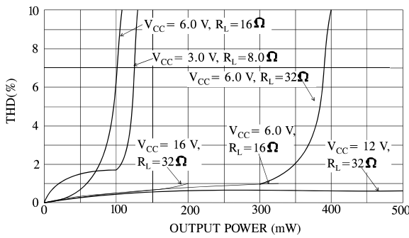
Figure 5. DISTORTION versus POWER f = 1.0 kHz, AVD = 34 dB
