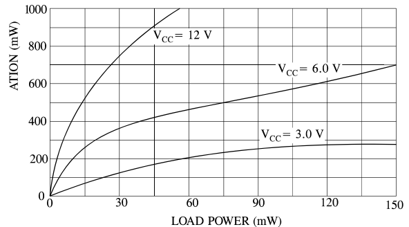
Figure 2. DEVICE DISSIPATION 8.0 \Omega LOAD
