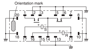
G6WK-1P
