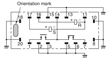
G6WK-1F
