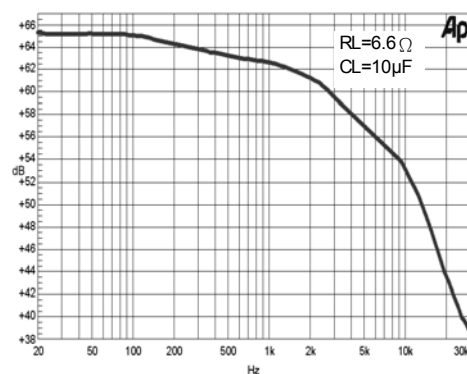
Power Supply Rejection Ratio
