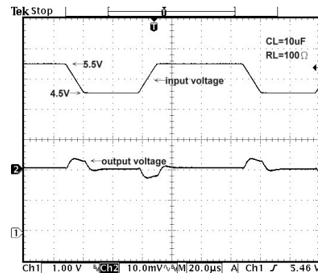
Line Transient
