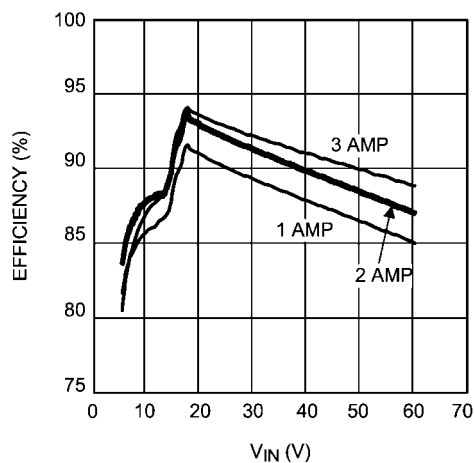
Efficiency vs V_{IN} and I_{OUT} V_{OUT} = 12V
