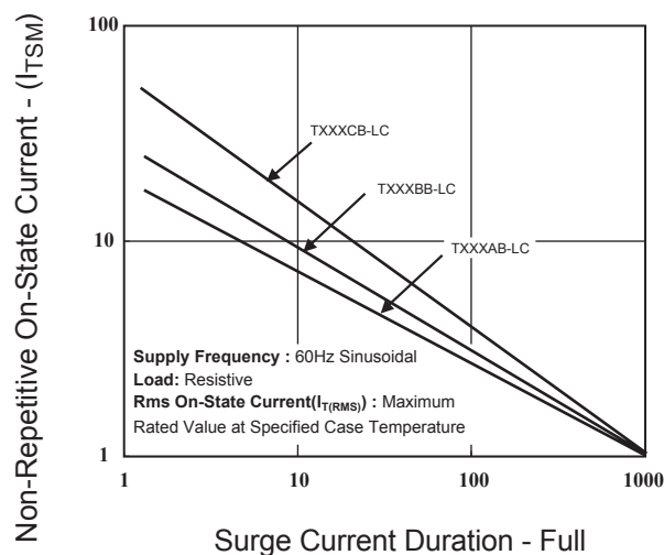
Fig.6 On-State Current Vs Surge Current
