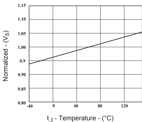
Fig.5 Typical normalized VS Vs Junction Temperature
