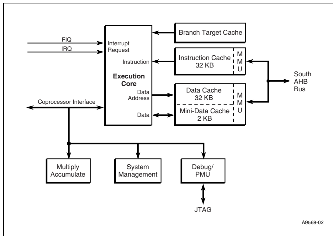
Figure 6. Intel XScale® Core Block Diagram
