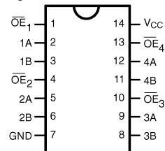
Pin Assignment for SOIC and TSSOP
