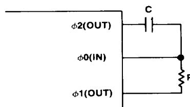
Suggested RC network configuration for internal oscillator.
