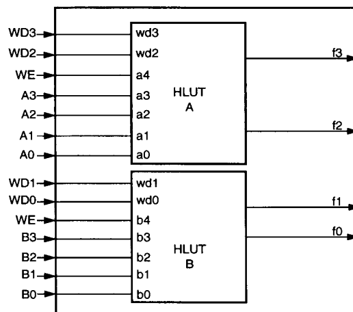
Figure 4. Dual 16 x 2 RAM/ROM
