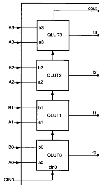
Figure 3. Ripple Mode
