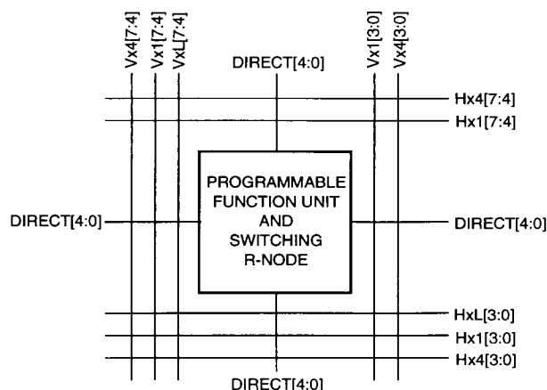
Figure 5. PLC Routing Resources
