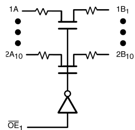
20-Bit Configuration
