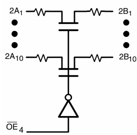
10-Bit Configuration
