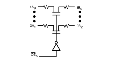
4-Bit Configuration
