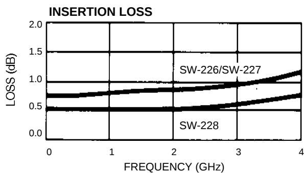
Typical Performance
