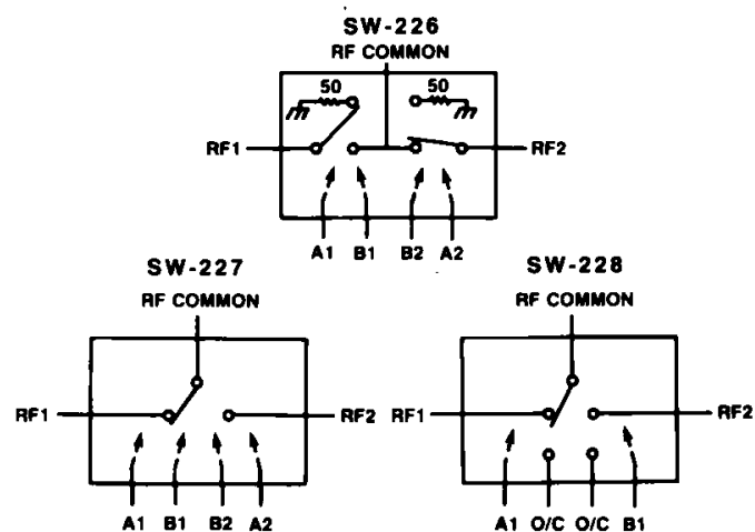
Pin Configuration
