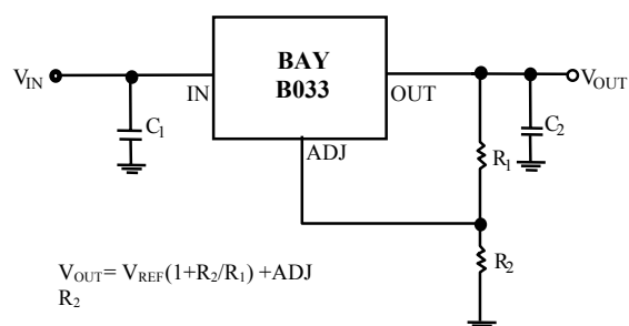
Typical Adjustable Regulator
