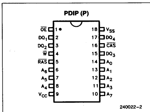
Figure 2. Pin Configuration
