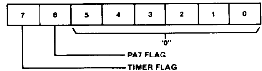
Figure 5. Interrupt Flag Register
