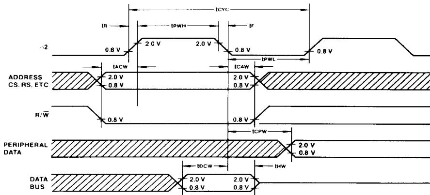
Figure 2. Write Timing
