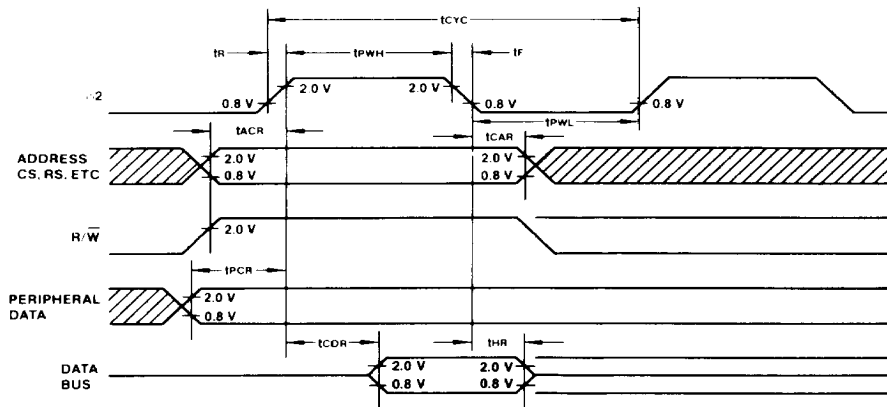
Figure 1. Read Timing
