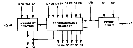
Figure 3. Basic Functions of Interval Timer
