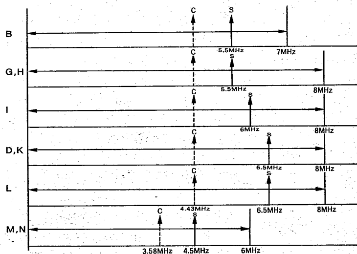
Comparison of Broadcasting Systems (Channel bandwidth and picture—sound bandwidth)
