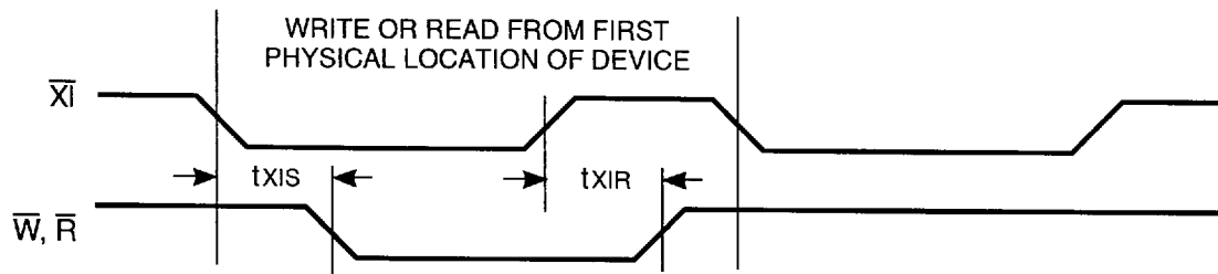
FIGURE 13. EXPANSION-IN TIMING
