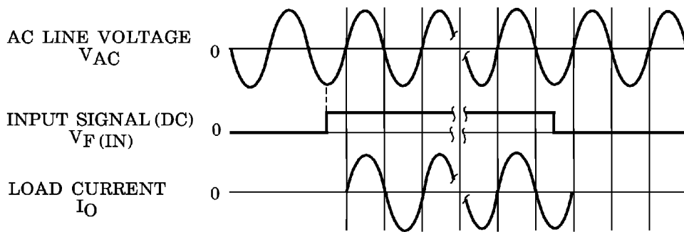
ZERO VOLTAGE SWITCHING WAVEFORM
