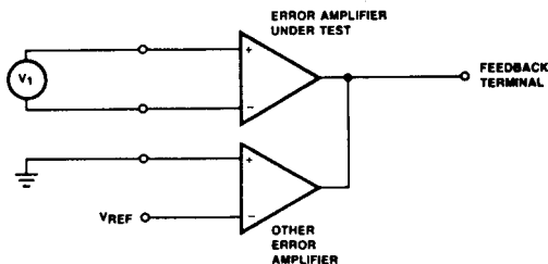
Figure 3. Error-Amplifier Characteristics
