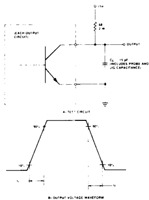
Figure 1. Common-Emitter Configuration
