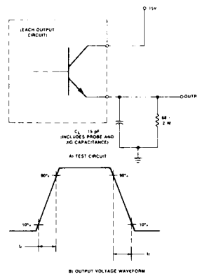
Figure 2. Emitter-Follower Configuration
