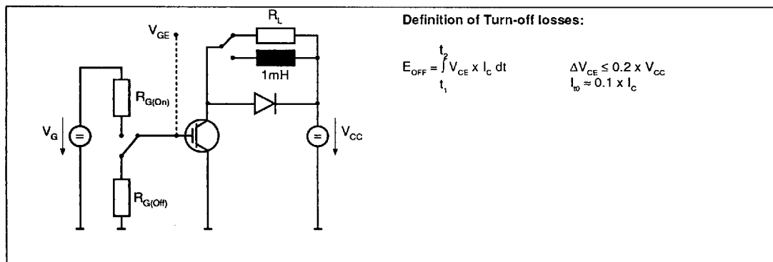
Fig.3 Test circuit
