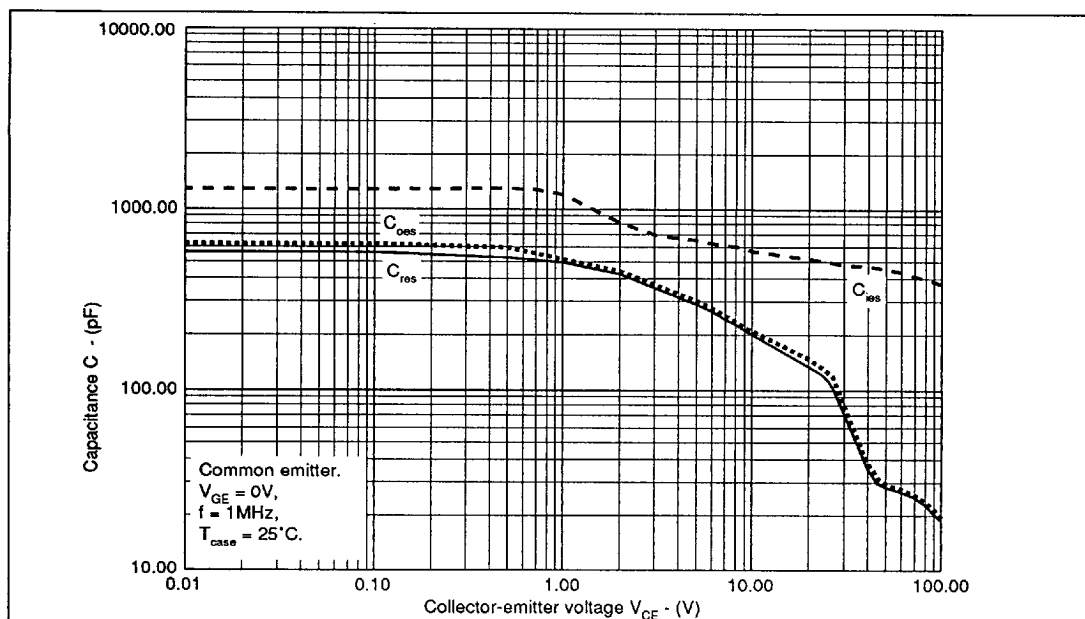
Fig.12 Typical capacitance
