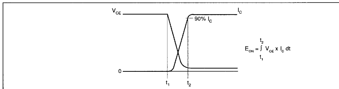
Fig.5 Definition of turn on losses
