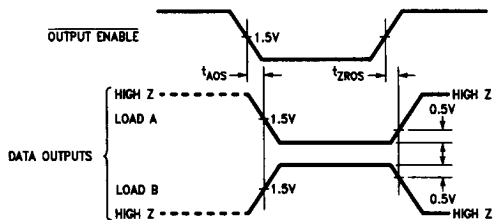
3c. Read Mode Propagation Delay from Output Enable
