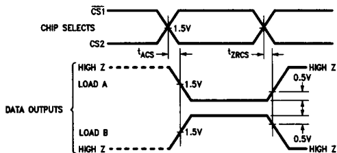
3b. Read Mode Propagation Delay from Chip Select
