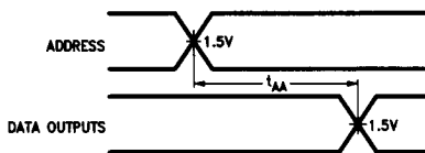
3a. Read Mode Propagation Delay from Address
