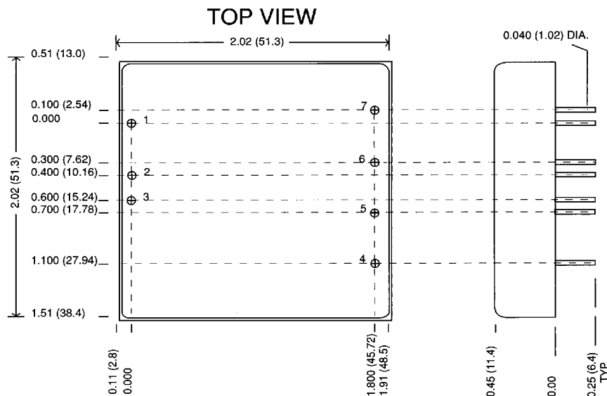
VPG SERIES CASE DRAWING NOMINAL CASE DIMENSIONS IN INCHES (MM) TOLERANCE X.XX ±0.02 (0.5), X.XXX ±0.005 (0.13)
