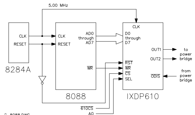
Fig. 5 8088 to IXDP610 Interface
