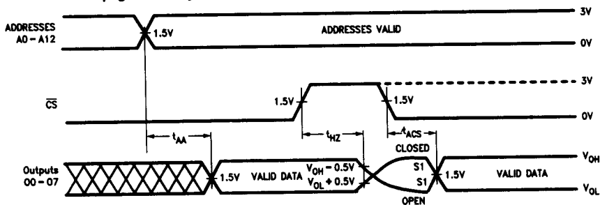
Propagation Delay from Address Valid to Output and \overline{\text{CS}} Valid to Output
