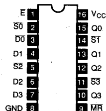
NTE8314 16-Lead DIP, See Diag. 249 4-Bit Latch
