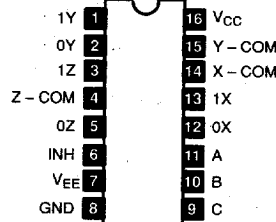
NTE74HC4053 16-Lead DIP, See Diag. 249 Triple 2-Channel Analog Multiplexer/Demultiplexer (CMOS)
