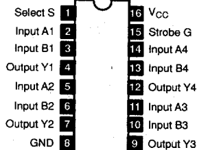
NTE8309 16-Lead DIP, See Diag. 249 Dual Selector/Multiplexer
