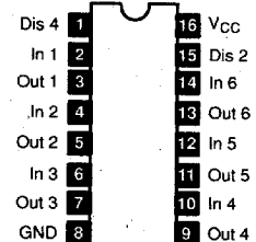
NTE80C95, NTE80C96, NTE80C97 16-Lead DIP, See Diag. 249 TRI-STATE Hex Buffer
