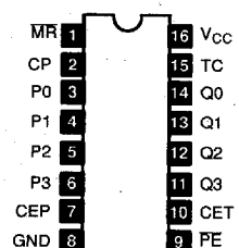
NTE8316 16-Lead DIP, See Diag. 249 Synchronous 4-Bit Binary Counter
