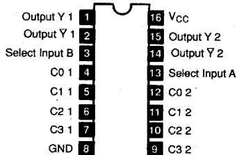
NTE8309 16-Lead DIP, See Diag. 249 Dual Selector/Multiplexer
