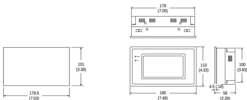
Panel Cutout
