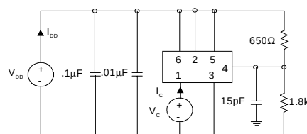
Figure 3. Output Test Conditions (25±5°C)
