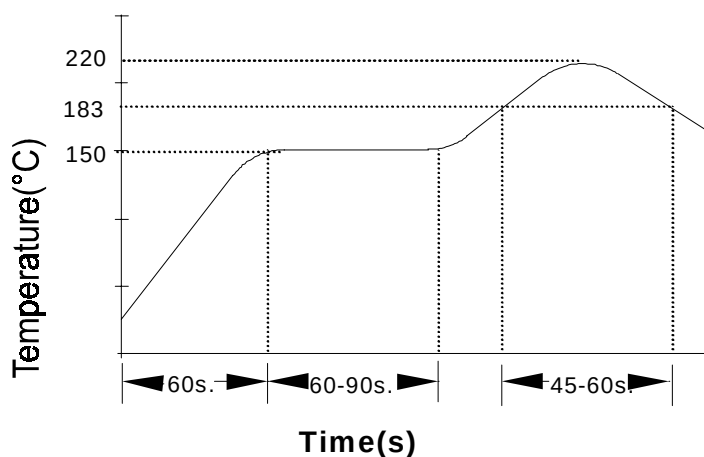
Figure 4. Suggested IR profile
