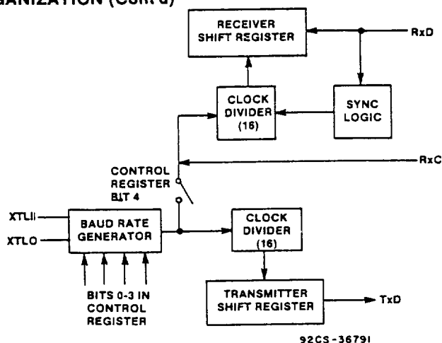
Fig. 6 - Transmitter receiver clock circuits.
