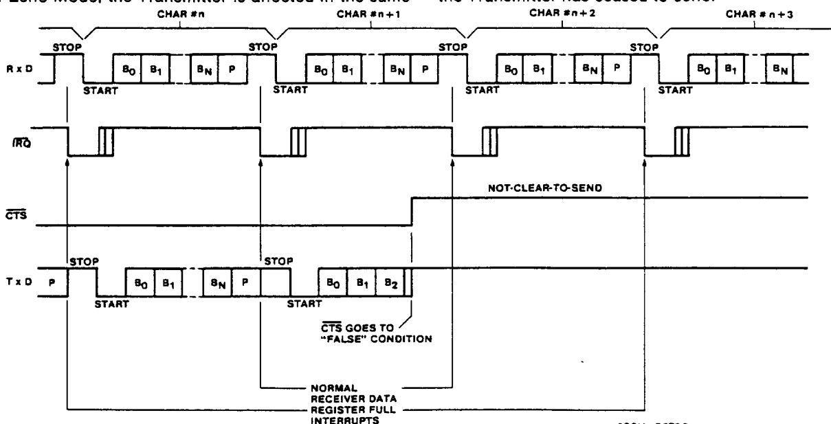
Fig. 13 - Effect of \overline{\text{CTS}} on echo mode.
