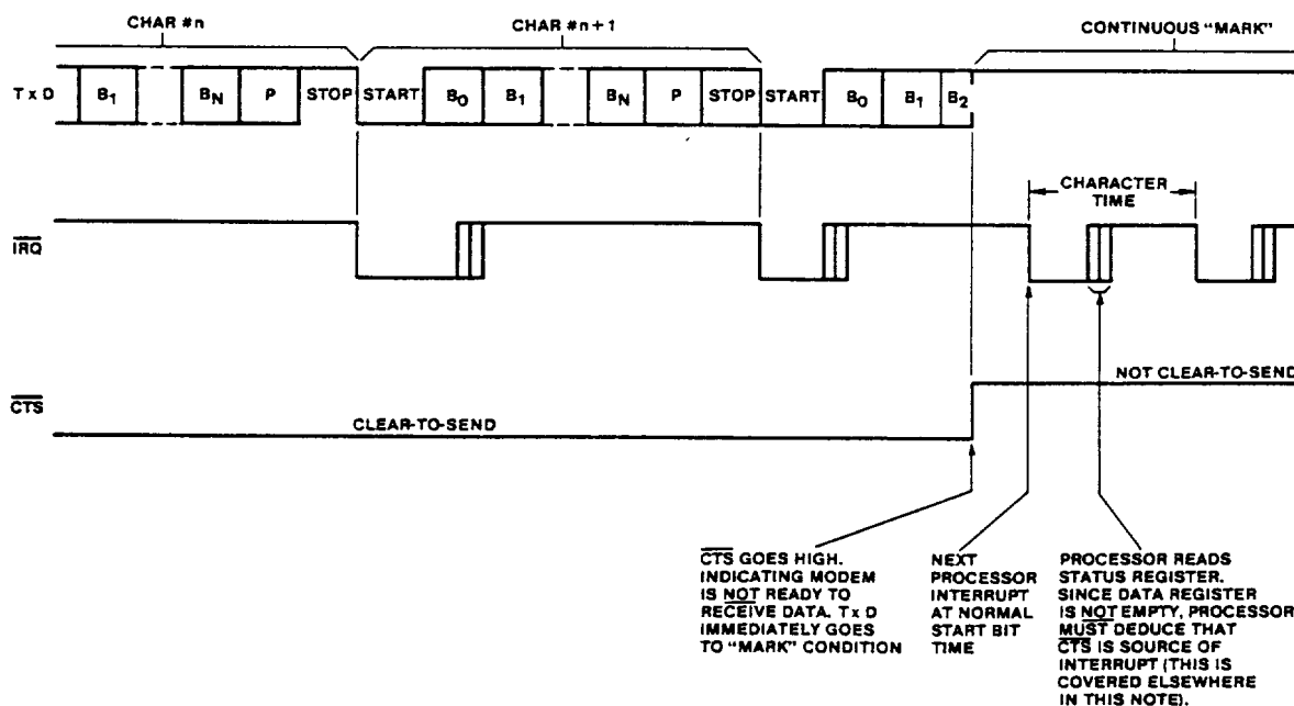
Fig. 10 - Effect of \overline{\text{CTS}} on transmitter.
