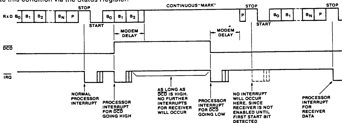
Fig. 16 - Effect of \overline{\text{DCD}} on receiver.
