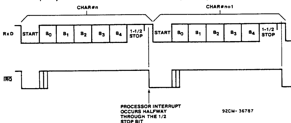
Fig. 17 - Timing with 1\frac{1}{2} stop bits.
