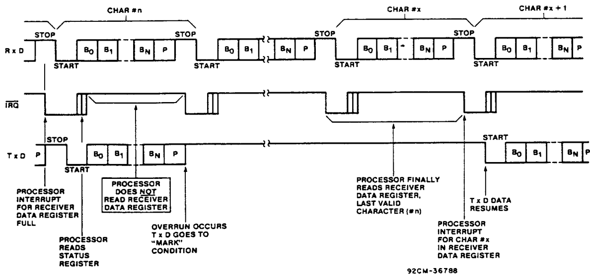
Fig. 14 - Overrun in echo mode.
