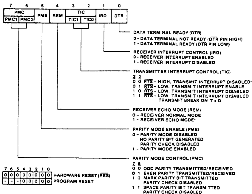
Fig. 5 - CDP65C51 command register.
