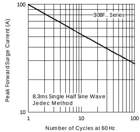
Fig. 4 - Max. Non-Repetitive Forward Surge Characteristic
