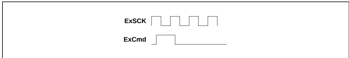
Figure 7. ExSIO Reset Sequence
