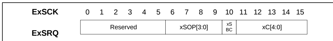
Figure 6. Expansion Bus Non-Register Operation Packet Format
