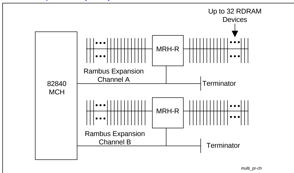
Figure 1. Intel® 840 Chipset Memory Subsystem with MRH-Rs
