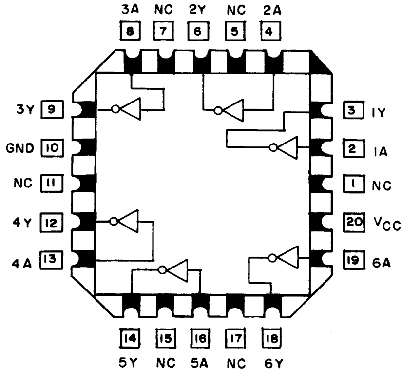
FIGURE 1. Logic diagram and terminal connections (top view).
