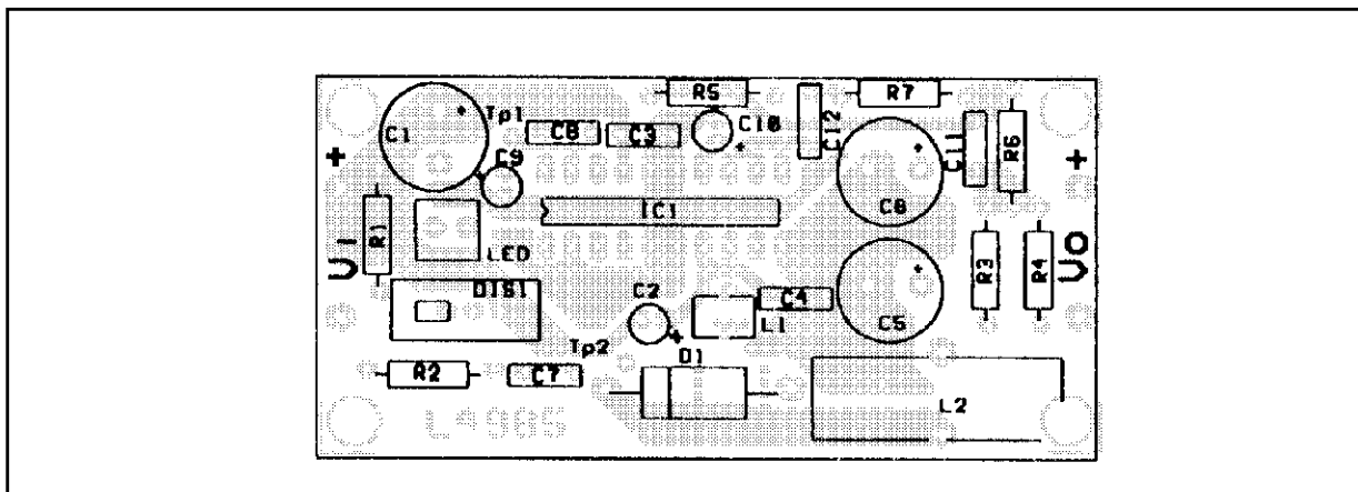
Figure 31: PC Board (Back Side) and Components Layout of Fig. 28 (scale 1:1)
