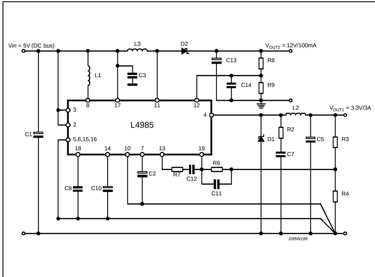
Figure 33 : Single chip converter generates 3.3V/3A for logic and 12V/100mA (flash eeprom) from 5V bus
