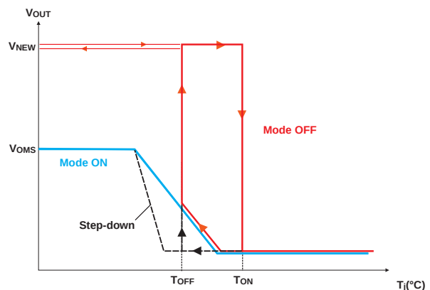
Fig. 12: Modified characteristics.
