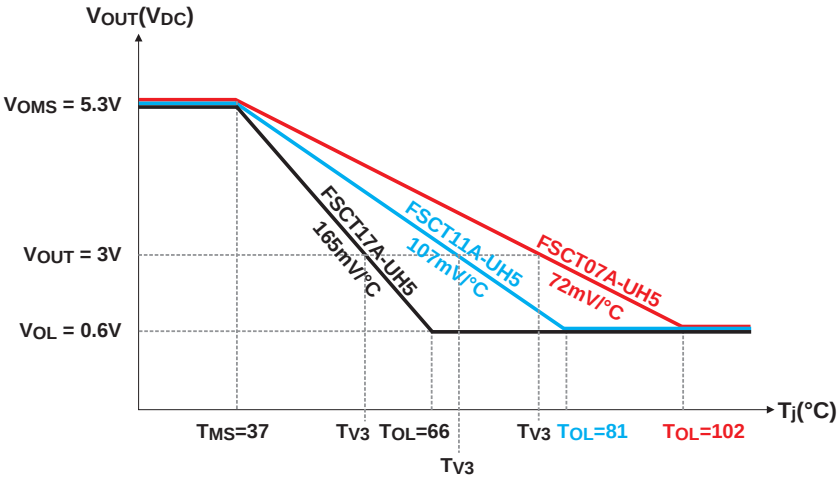
Fig. 3: Temperature slopes.
