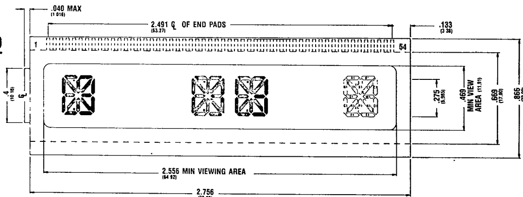
PINOUT: #350
