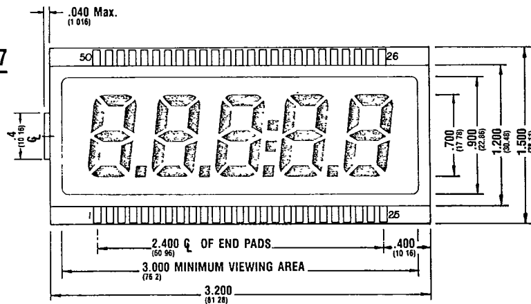
PINOUT: #57
