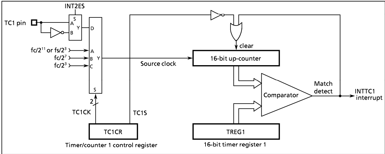
Figure 2-16. Timer/Counter 1
