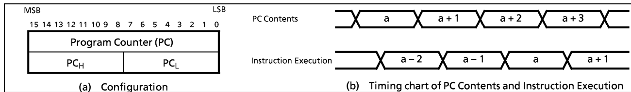
Figure 1-3. Program Counter
