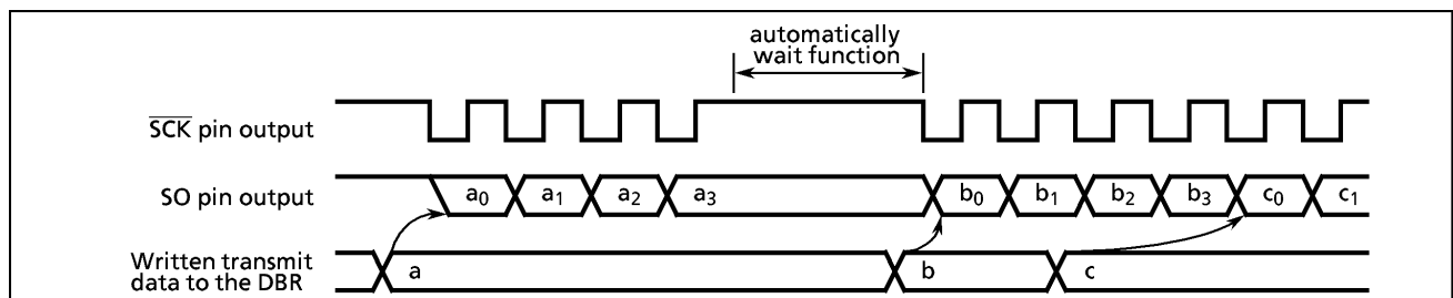
Figure 2-31. Clock Source (Internal Clock)
