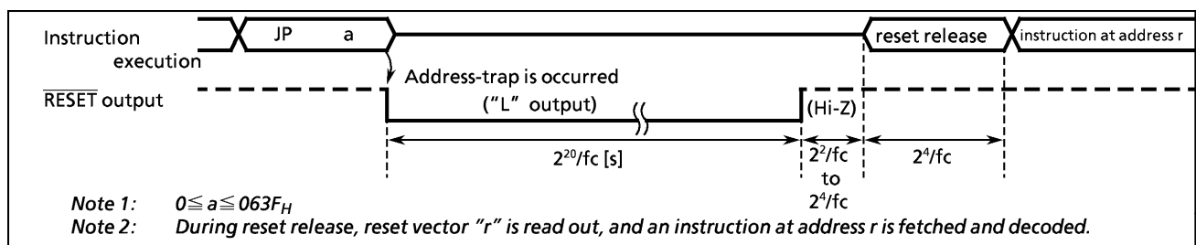
Figure 1-31. Address-Trap-Reset
