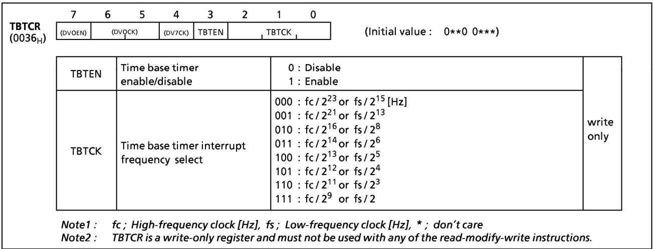
Figure 2-13. Time Base Timer and Divider Output Control Register
