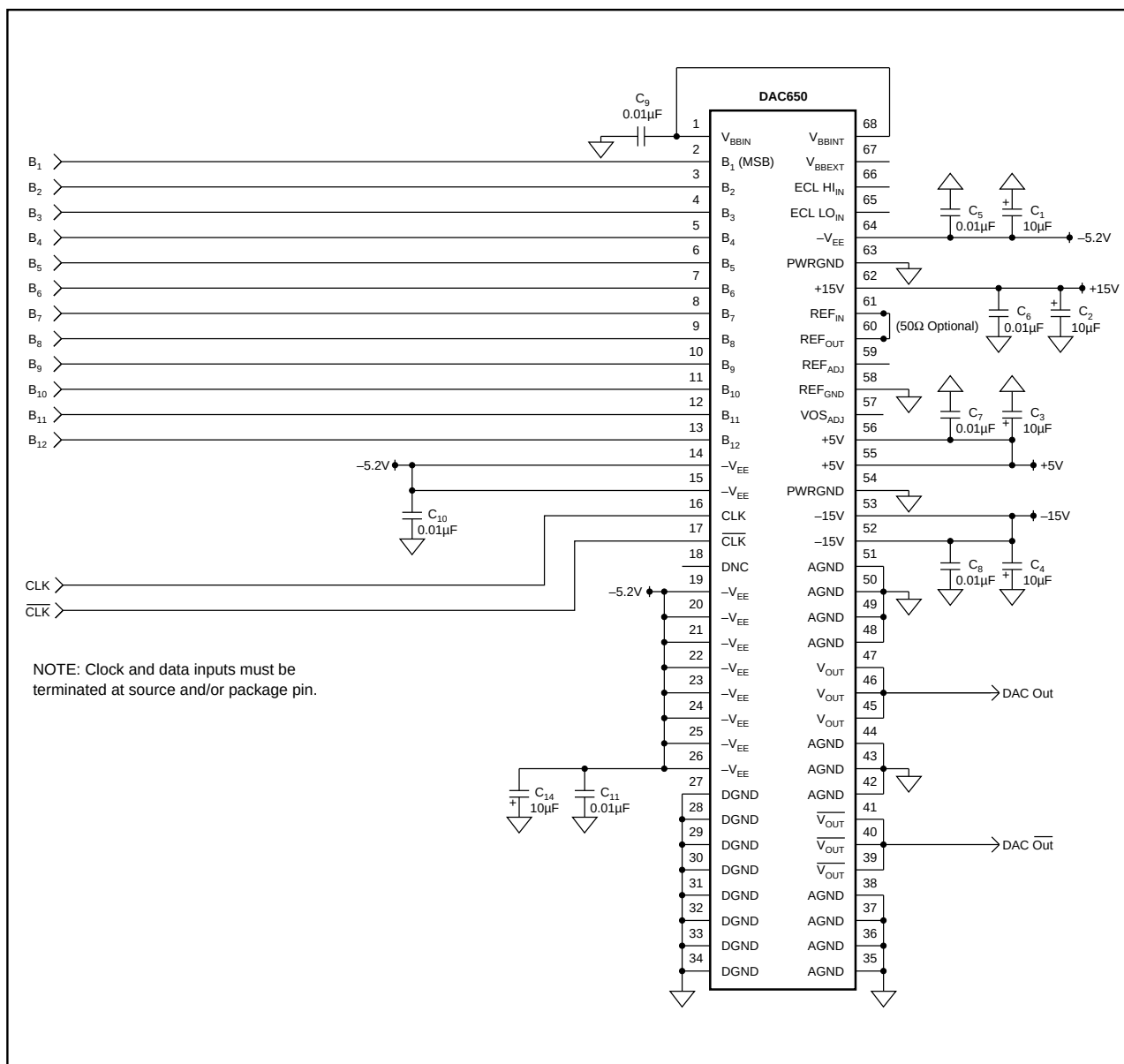
FIGURE 8. Typical DAC650 Connection Diagram.
