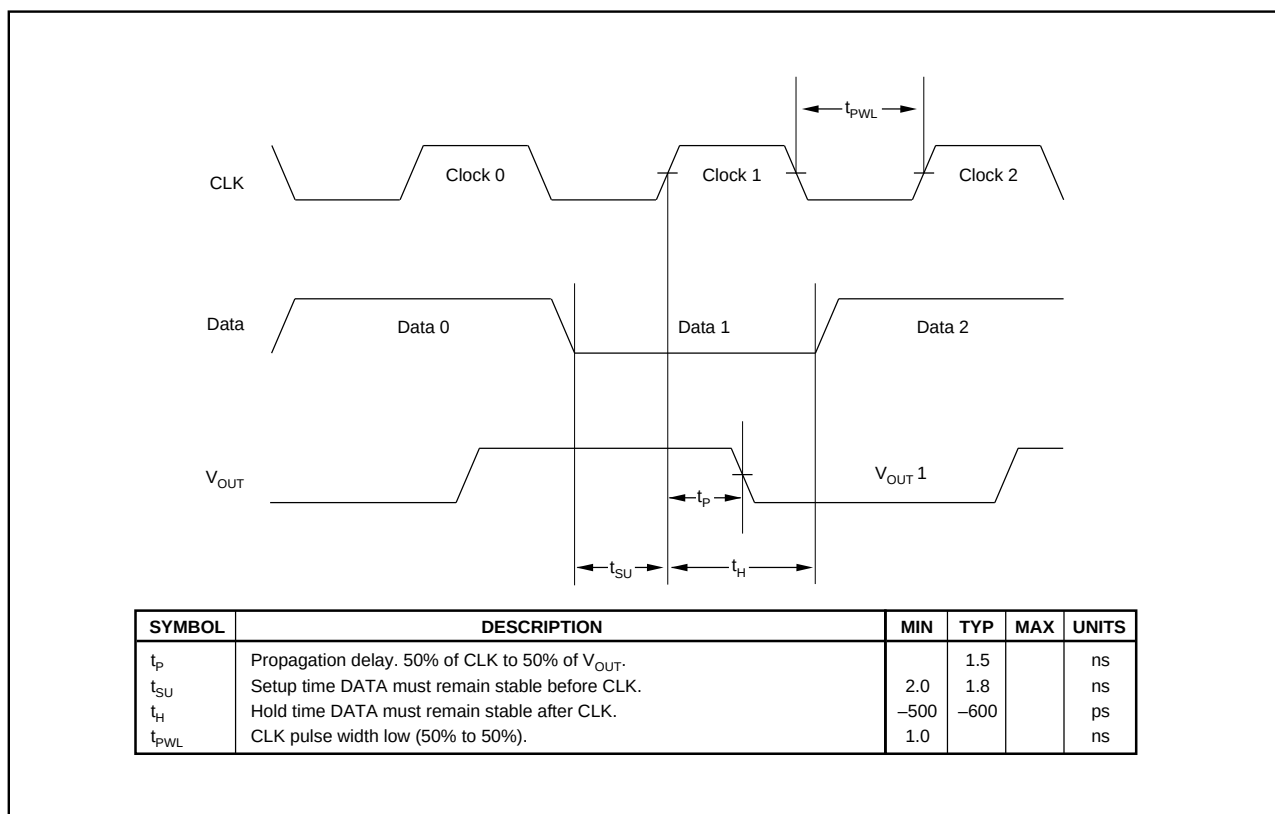
FIGURE 4. Timing Diagram for the DAC650.
