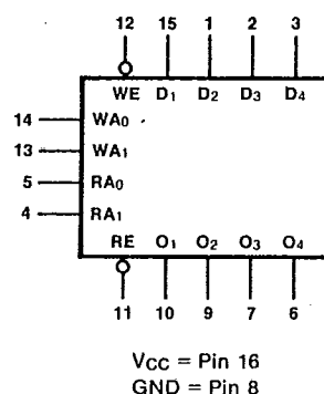
LOGIC SYMBOL
